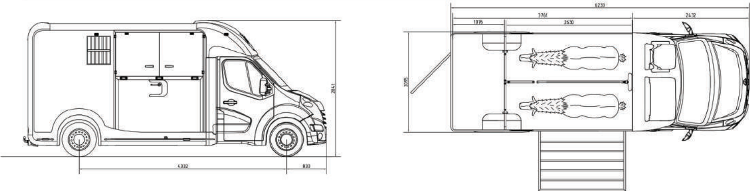
CABINE SIMPLE - VERSION HARAS
