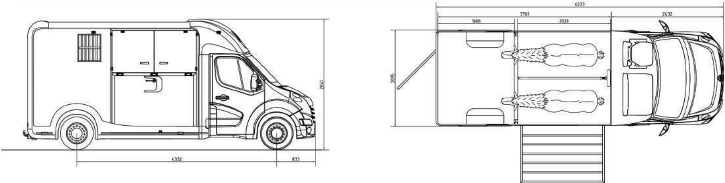
CABINE SIMPLE - VERSION STANDARD
